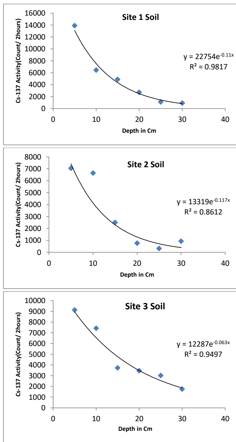
Fig .6: Exponential regression of Cs-137 activity as function of soil depth at location A.
