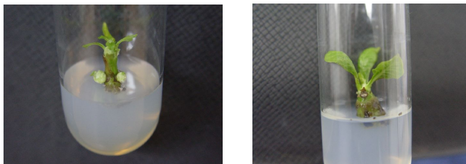
Shape (1): Shoots initiation of Gardenia jasminoides on MS medium supplemented with BA+IAA at different concentrations after 4-6 weeks of culture.
