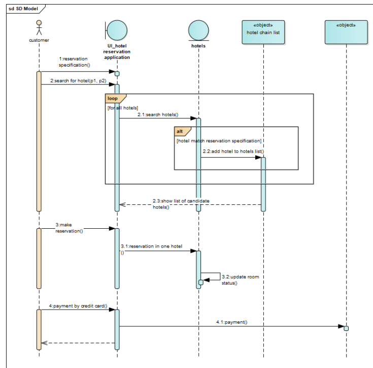
Figure 2: SD1 version 1 for hotel reservation system.
