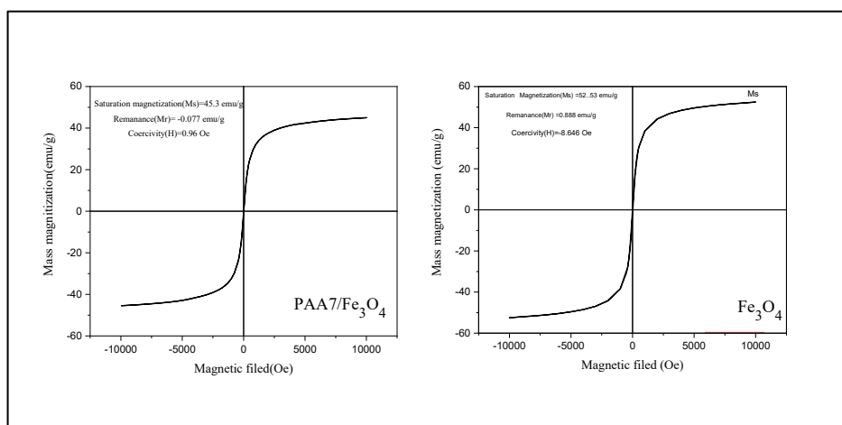
Figure 4 . Magnetic moment loop of \text{Fe}_3\text{O}_4 and \text{AC}/\text{Fe}_3\text{O}_4
