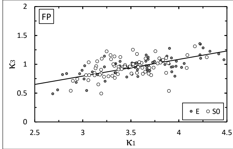
Figure 3. The FP in \kappa space
