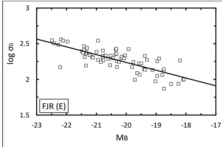
Figure 4. The FJR of E galaxies
