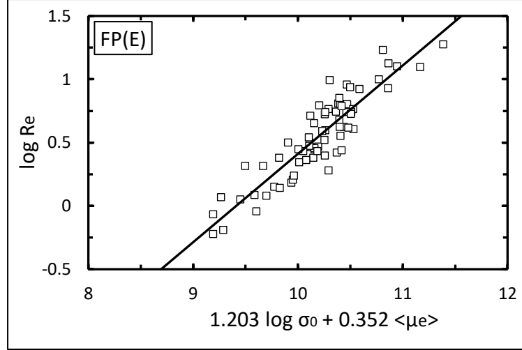
Figure 1. The FP for E galaxies
