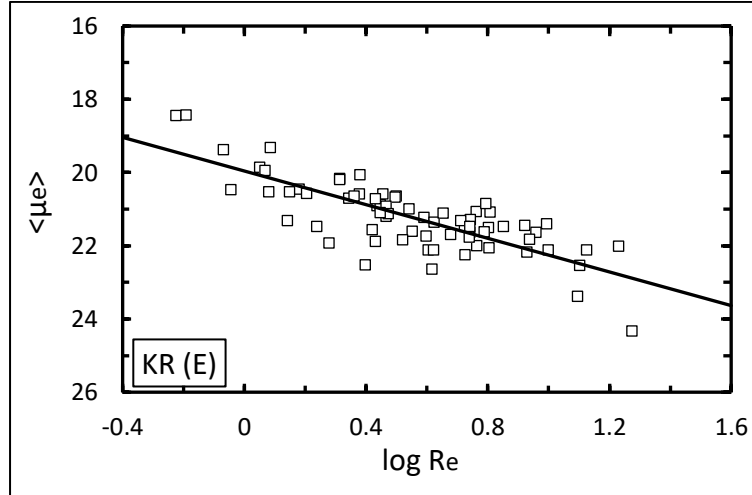
Figure 6. The KR of E galaxies
