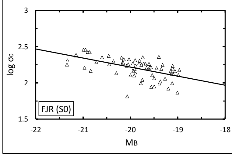
Figure 5. The FJR of S0 galaxies
