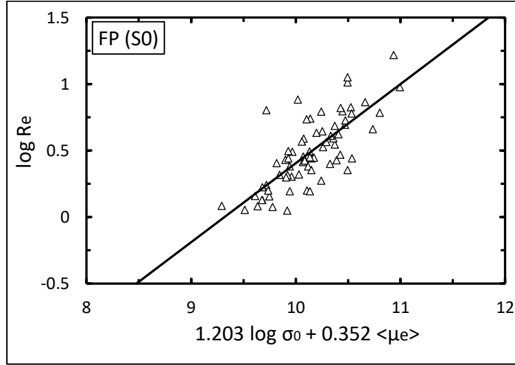
Figure 2. The FP for S0 galaxies
