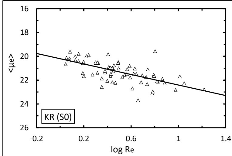
Figure 7. The KR of S0 galaxies
