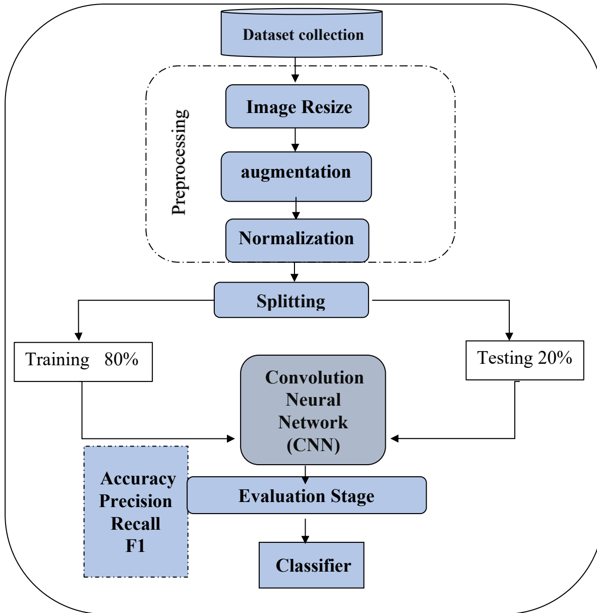
Figure2. A flowchart of the suggested method for detecting Alzheimer's disease at an early stage.
