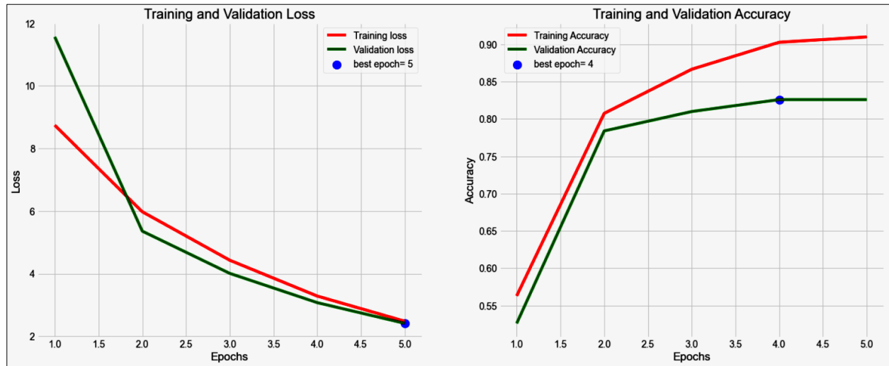
Figure 4: Losses ratio of ResNet50 model.
