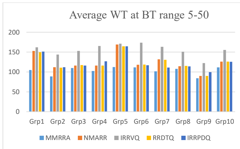
Figure 6. Average waiting times at burst time range of 5-50
