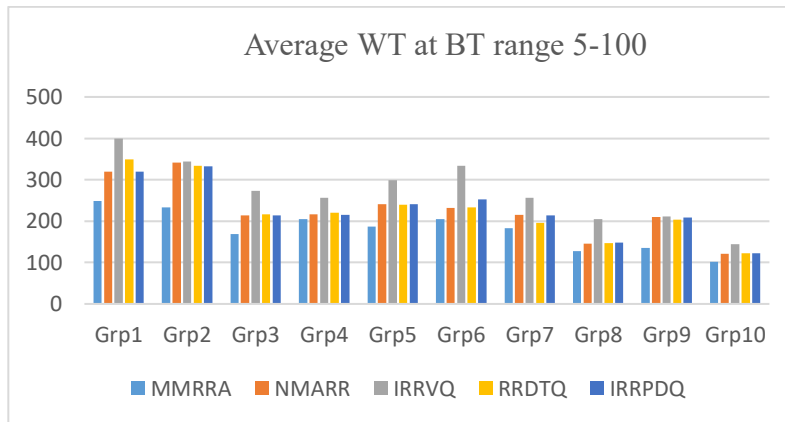
Figure 7. Average waiting times at burst time range of 5-100
