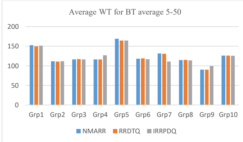
Figure 2. Average waiting times at burst time range of 5-50
