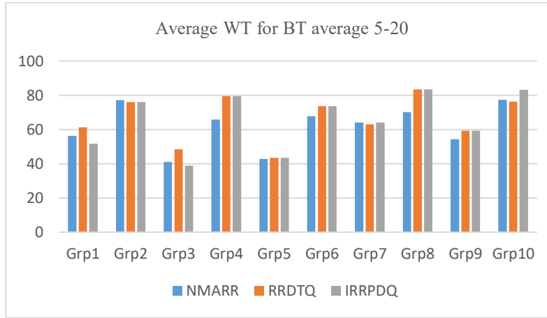
Figure 1. Average waiting times at burst time range of 5-20
