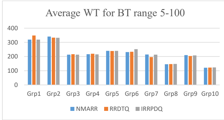
Figure 3. Average waiting times at burst time range of 5-100
