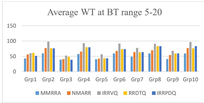
Figure 5. Average waiting times at burst time range of 5-20
