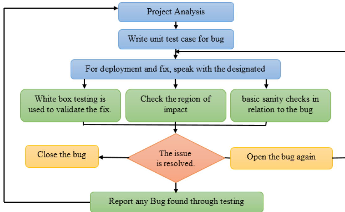
Figure 2. Manually executing tests
