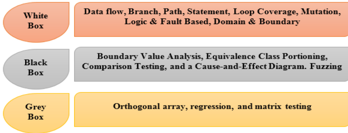
Figure 1. Dynamic Testing Techniques
