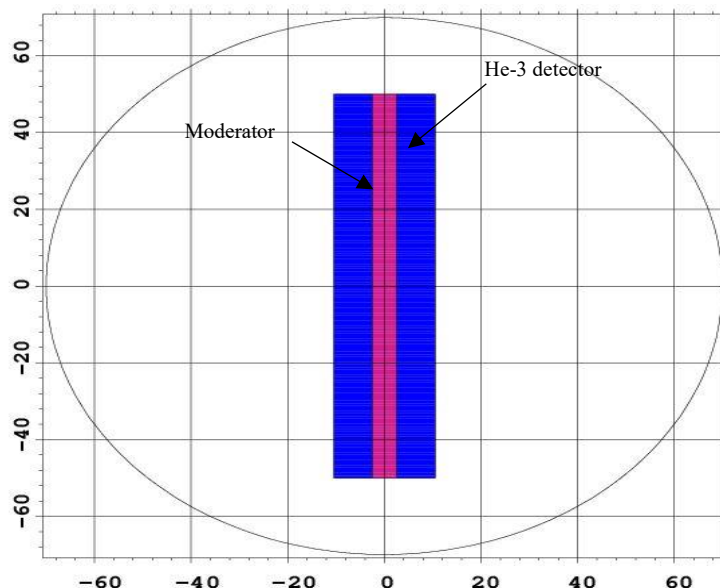
Figure 3. Schematic diagram of the MCNPX 6.2-modeled ^3\text{He} detector in xy plane.
