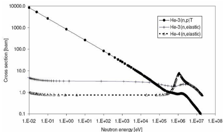
Figure 1. Neutron capture cross-section [3]
