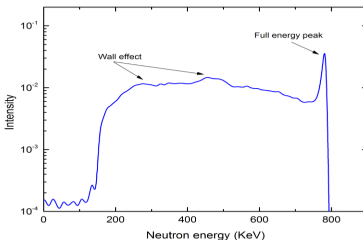
Figure 5. Pulse height spectrum of the ^3\text{He} detector
