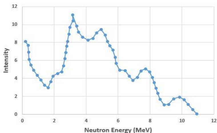
Figure 2. Am-Be neutron source energy spectrum [17]
