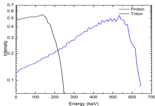
Figure 4. The distribution of proton and triton energy
